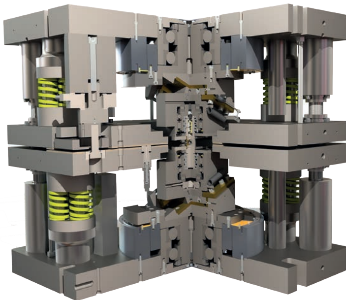
Fig. [2] Tool for hole-rolling on conventional servomotor presses
