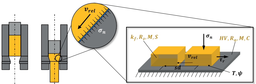
Fig. [2] Tribological system in cold forging
