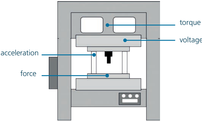
Fig. [1] Data acquisition in production through sensor integration
