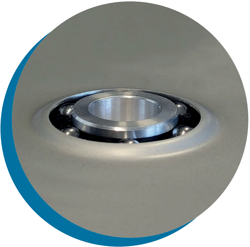
Fig. [3] Integrated bearing with hole-rolled outer race
