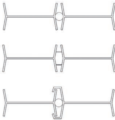
Fig. [1] Possible bearing designs
